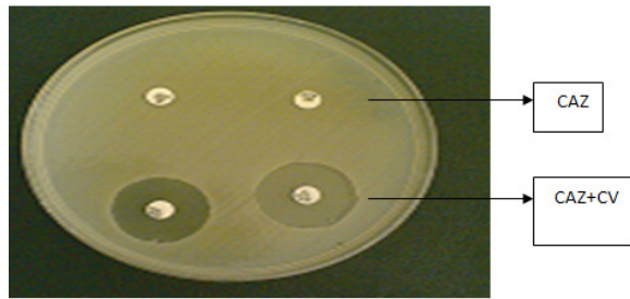
Figure 2. Phenotypic Test for ESBL-Positive Isolates.
